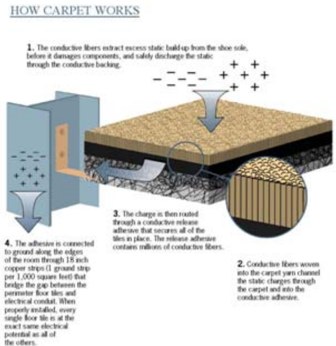
Figure 1: ESD CARPET
